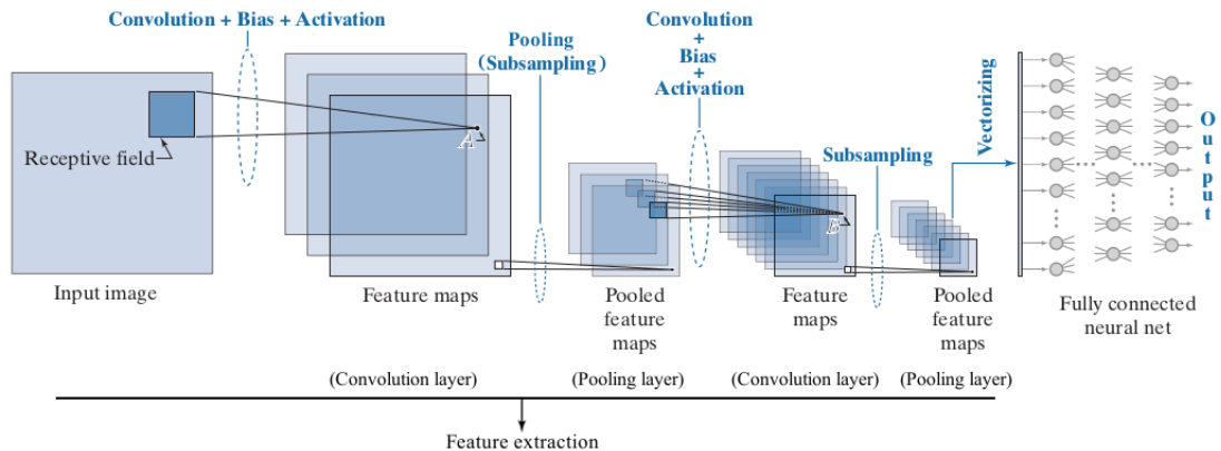
Figure 2.4: A simple CNN with LeNet architecture.[11, altered]
