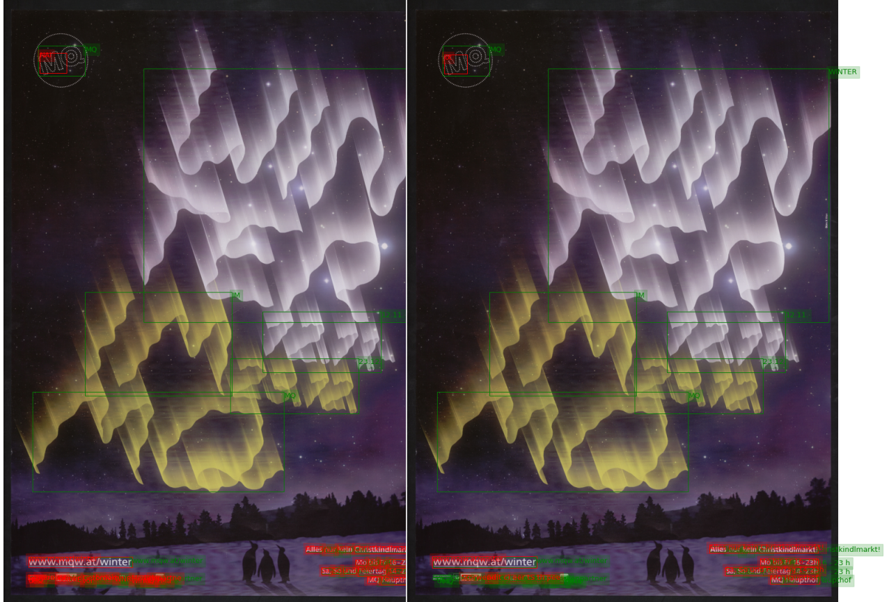
(a) EasyOCR
