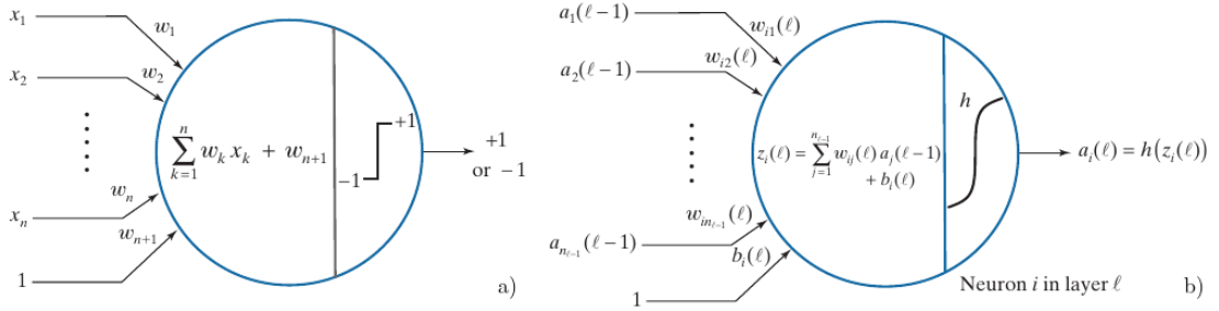
Figure 2.1: Model of a perceptron unit (a), model of an artificial neuron (b) with used operations. The letter h denotes an activation function, l denotes a particular layer in a multilayer network. The element on the right is sometimes called a sigmoid neuron.[11]
