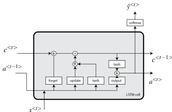
Figure 2.5: Scheme of a LSTM recurrent neural network.[39]
