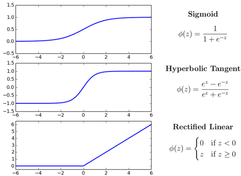
Figure 2.2: Commonly used activation functions in neural networks.[13, altered]
