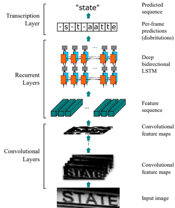
Figure 2.6: An architecture of CRNN for recognizing objects in images.[30]
