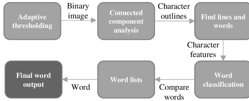
Figure 3.1: Pipeline architecture of Tesseract OCR engine. [10]
